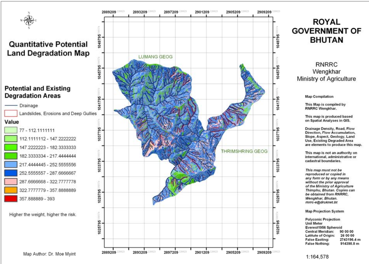
Figure 2. Quantitative Potential Land Degradation Map.
