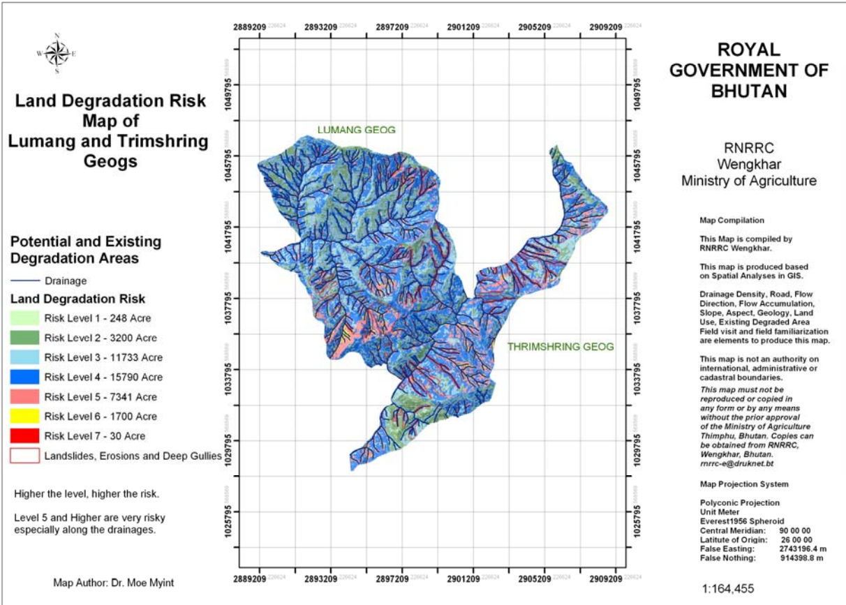
Figure 3. Land Degradation Risk Map.
