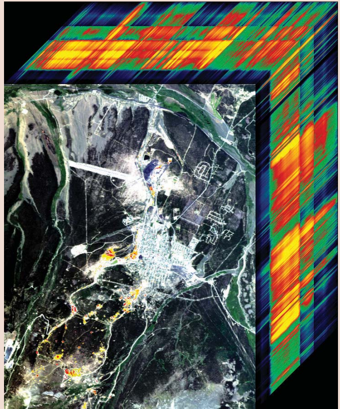
Hyperspectral images are sometimes referred to as “image cubes” because they have a large spectral dimension as well as the two spatial dimensions. This cube shows an AVIRIS hyperspectral image of the Leadville mining district in Colorado, with the spectral dimension shown as the top and right faces of the cube. The front of the cube is a true color composite, with areas containing secondary minerals from acid mine drainage highlighted in red, orange and yellow. This cube was processed using ENVI.
