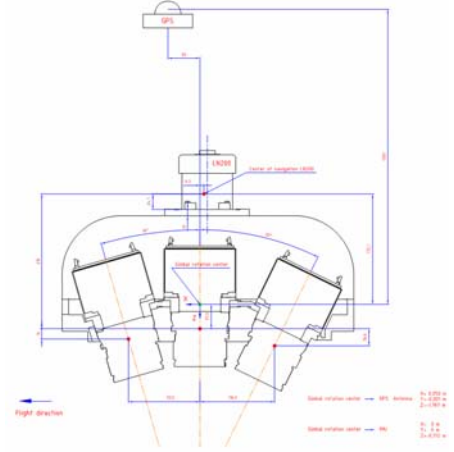
Figure 1. Sensor design.
