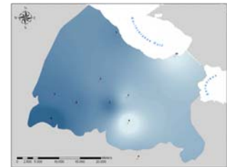
Figure 3. Distribution of monthly precipitation (range: 48-113 mm)
