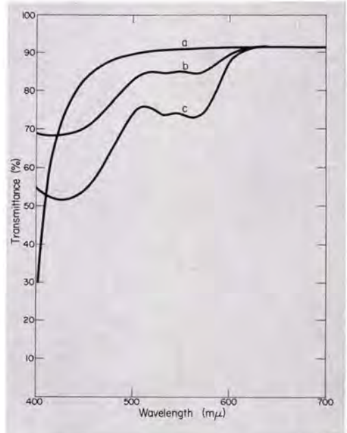
FIG. 6. Transmittance characteristics of (a) the Kodak Wratten Filter No. 2B, (b) Kodak Haze Filter, HF-4, and (c) HF-5.
