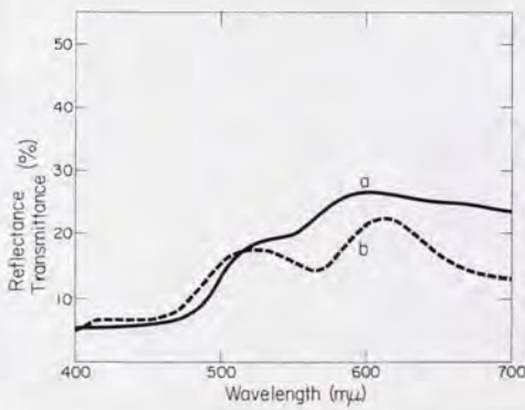
FIG. 3. Spectral reflectance curve (a) of a dark yellow sample, and spectral transmittance curve (b) of a typical photographic reproduction in a reversal color film.
