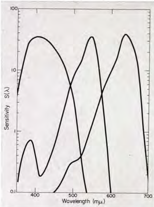
FIG. 1. Spectral sensitivity of Kodak Ektachrome MS Aerographic Film (Estar Base), Type SO-151. S(\lambda) = E(\lambda)^{-1} , where E(\lambda) is the energy in ergs·Cm -2 of monochromatic radiation of wavelength \lambda required to reduce the dye image density in the individual layer to an equivalent neutral density of 1.0 above minimum density. Data are adjusted to correspond to an effective exposure time of 1/50 second.
