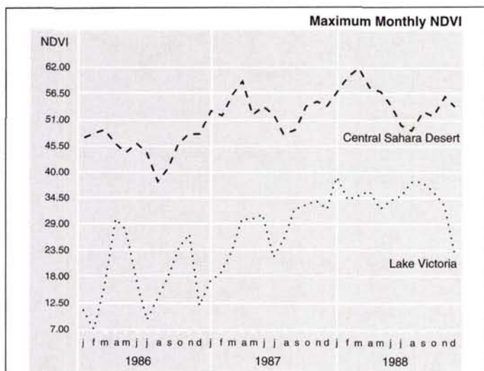
Figure 3. Time series profiles of monthly NDVI for sites in the central Sahara Desert and Lake Victoria, January 1986 to December 1988.
