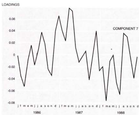
Figure 1. Loadings (Y-axis) of the original monthly images (X-axis) on the first eight standardized principal components. Loadings can equally be thought of as the correlation between the original images and the derived components.
